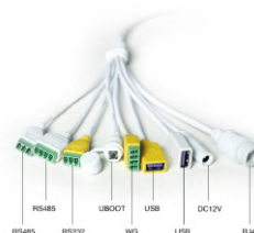
Communication module
